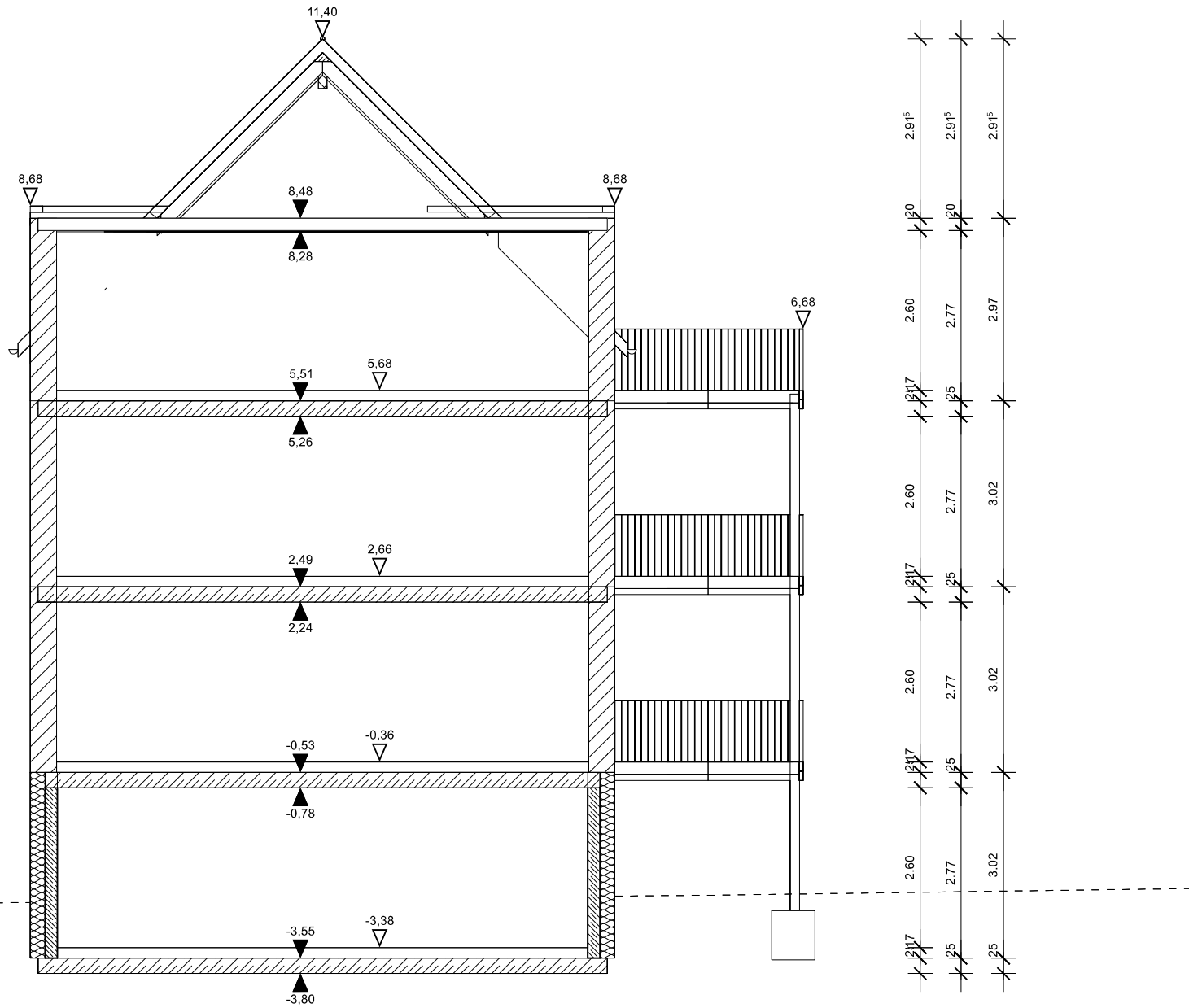
Schitt B-B
